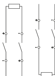
Wiring example miniature circuit-breakers DLS 6hdc C16-2
