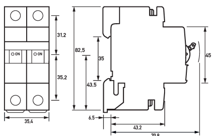
Dimensioned drawing miniature circuit-breakers DLS 6hdc C5-2
