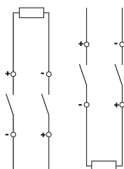
Wiring example miniature circuit-breakers DLS 6hdc C5-2
