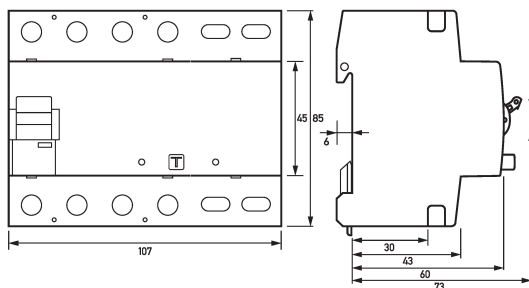
Dimensioned drawing switch-disconnectors DHS 6-063 NUS
