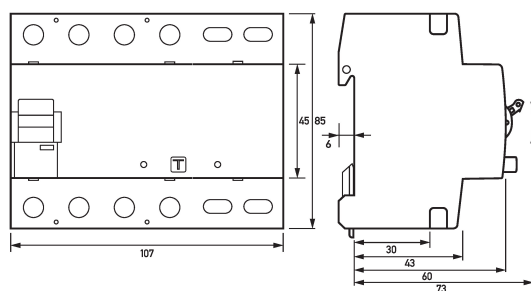
Dimensioned drawing switch-disconnectors DHS 6-o63 NU
