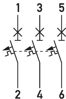
Wiring diagram DLS 6i, B-characteristic, threepole, 6kA
