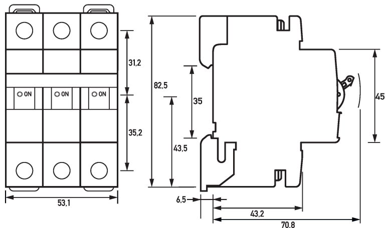
Dimensional drawing DLS 6i, B-characteristic, threepole, 6kA (Group view)
