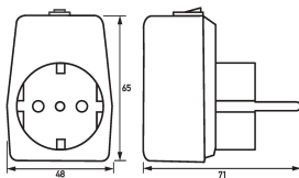
Dimensional drawing Group view
