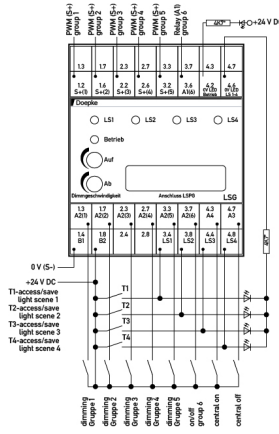
Wiring diagram
