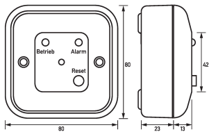
Dimensional drawing Group view
