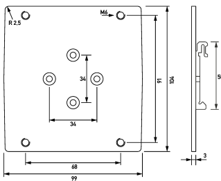
Dimensional drawing Group view
