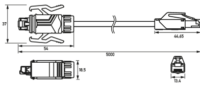
Dimensional drawing Group view
