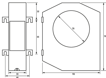
Dimensional drawing Group view
