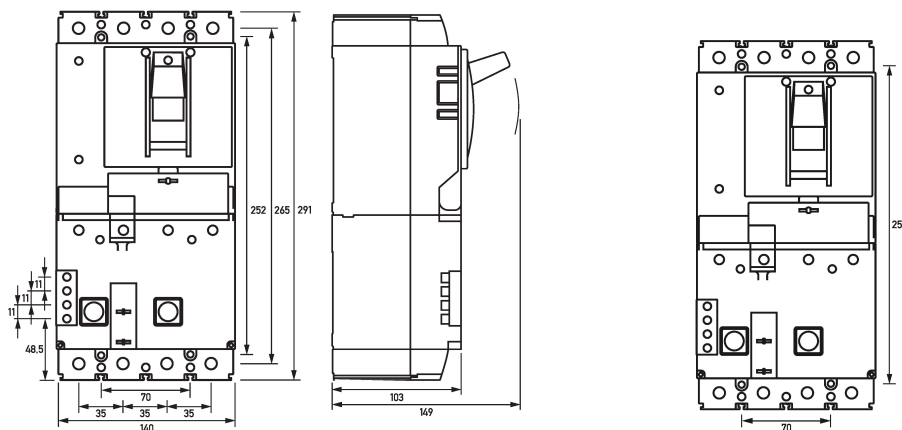
Dimensioned drawing circuit-breakers with residual current trip DFL 8 250-4/0,03-A
