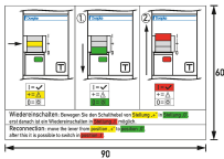
Dimensional drawing Group view
