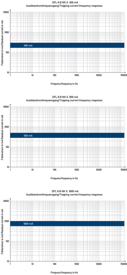
Characteristic B NK X 300 mA
