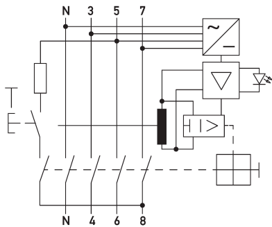
Wiring example residual current circuit-breaker DFS4 125-4/0,50-B SK S HD
