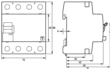
Dimensioned drawing residual current circuit-breaker DFS4 125-4/0,50-B SK S HD
