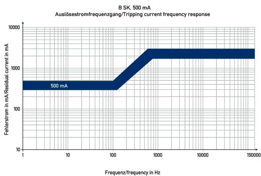
Diagrams residual current circuit-breaker DFS4 125-4/0,50-B SK S HD
