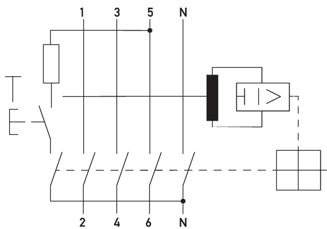
Wiring diagram DFS 4 A, 4-pole N right
