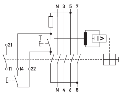
Wiring diagram
