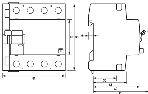
Dimensioned drawing residual current circuit-breaker DFS 4 125-4/0,03-AC FT
