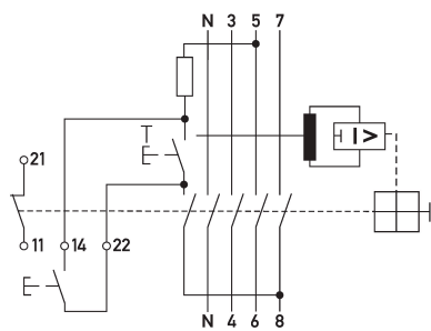
Wiring example residual current circuit-breaker DFS 4 125-4/0,03-AC FT
