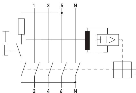
Wiring example residual current circuit-breaker DFS 4 100-4/0,30-AC R S
