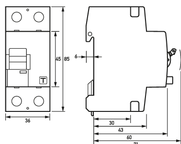
Dimensioned drawing residual current circuit-breaker DFS 2 080-2/0,50-A S
