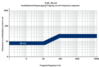
Characteristic B NK 100 mA
