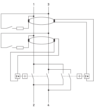
Wiring diagram
