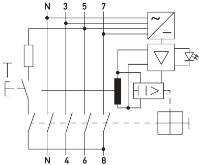
Wiring example residual current circuit-breaker DFS 4 063-4/0,50-B SK S V500
