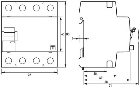
Dimensioned drawing residual current circuit-breaker DFS 4 063-4/0,50-B SK S V500
