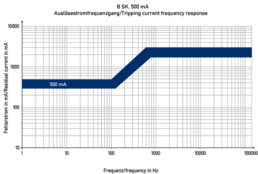
Diagrams residual current circuit-breaker DFS 4 063-4/0,50-B SK S V500
