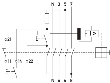
Wiring example residual current circuit-breaker DFS 4 063-4/0,50-A S FT
