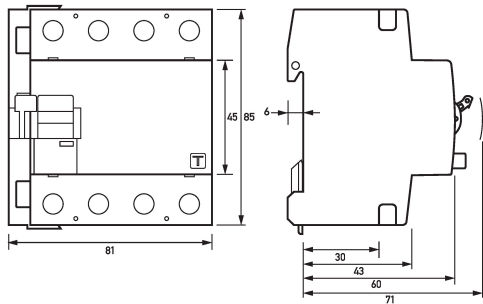
Dimensioned drawing residual current circuit-breaker DFS 4 063-4/0,50-A S FT
