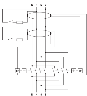
Wiring diagram
