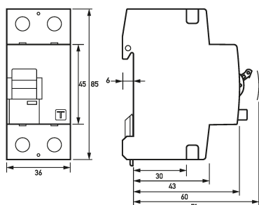
Dimensioned drawing residual current circuit-breaker DFS 2 063-2/0,50-A KV
