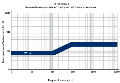
Characteristic B NK 100 mA
