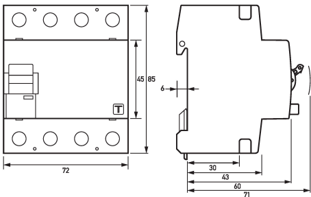
Dimensioned drawing residual current circuit-breaker DFS 4 063-4/0,10-B SK Hz60 HD
