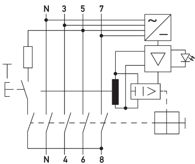
Wiring example residual current circuit-breaker DFS 4 063-4/0,10-B SK Hz60 HD
