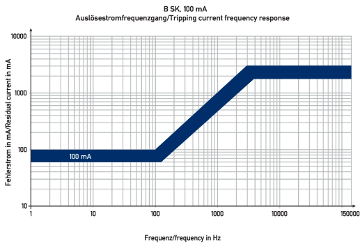
Diagrams residual current circuit-breaker DFS 4 063-4/0,10-B SK Hz60 HD
