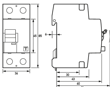
Dimensioned drawing residual current circuit-breaker DFS 2 063-2/0,10-AC
