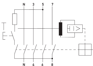
Wiring diagram
