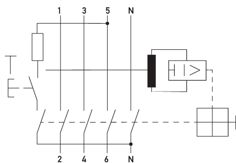
Wiring example residual current circuit-breaker DFS 4 063-4/0,03-AC R
