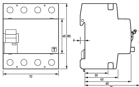
Dimensioned drawing residual current circuit-breaker DFS 4 063-4/0,03-B+ MI HD
