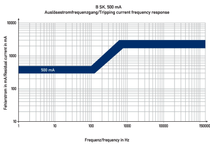
Characteristic B SK 500 mA
