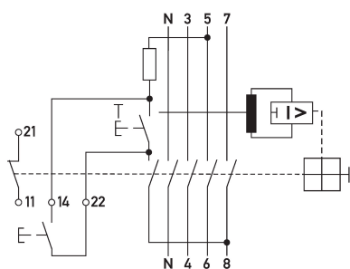
Wiring example residual current circuit-breaker DFS 4 040-4/0,30-A V500 FT
