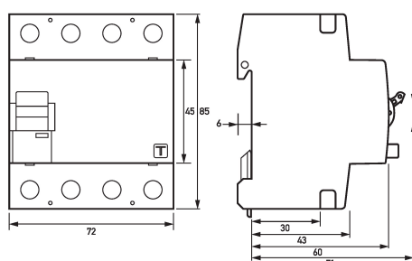
Dimensioned drawing residual current circuit-breaker DFS 4 040-4/0,30-A V110/190
