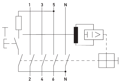
Wiring example residual current circuit-breaker DFS 4 A HD, 4-pole
