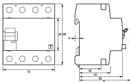
Dimensioned drawing residual current circuit-breaker DFS 4 A HD, 4-pole
