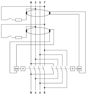
Wiring diagram
