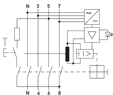
Wiring example residual current circuit-breaker DFS 4 040-4/0,30-HP HD
