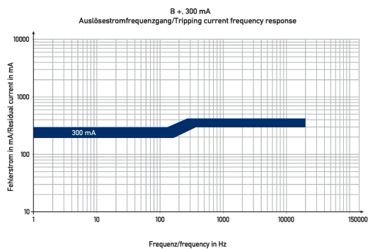
Diagrams residual current circuit-breaker DFS 2 040-2/0,30-B+ HD
