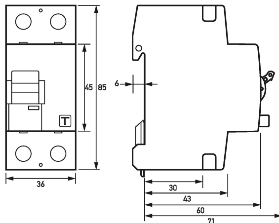
Dimensional drawing DFS 2 HP, 2-pole (Group view)
