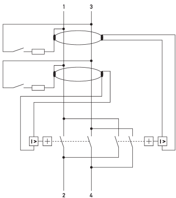
Wiring diagram
