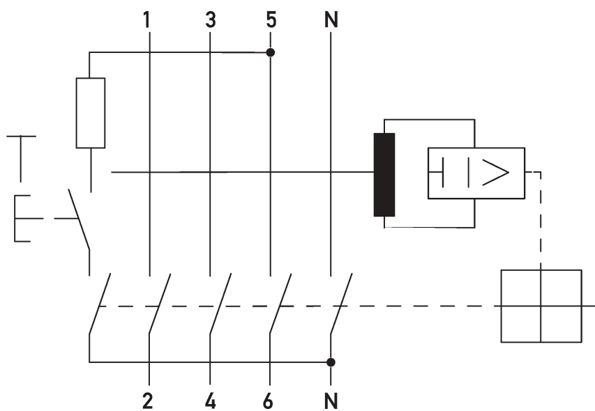
Wiring diagram DFS 4 A KV, 4 pole N right
