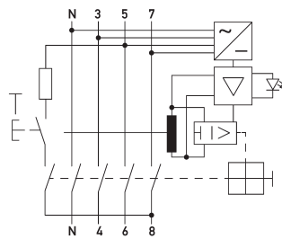
Wiring diagram
