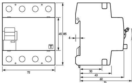
Dimensional drawing Group view
