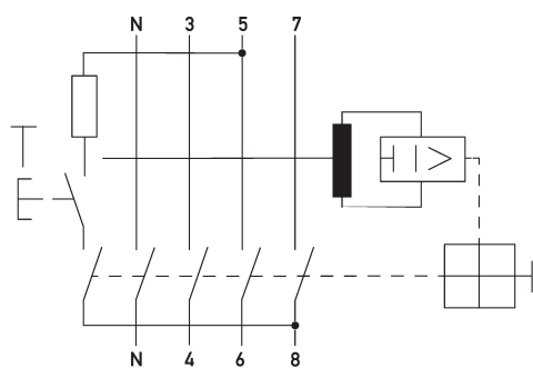
Wiring example residual current circuit-breaker DFS 4 040-4/0,03-AC Hz60
