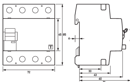
Dimensioned drawing residual current circuit-breaker DFS 4 040-4/0,03-AC Hz60
