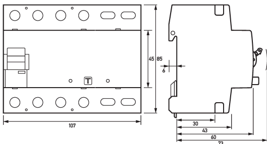
Dimensional drawing Group view
