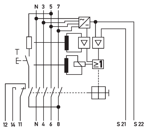
Wiring diagram DFS 4 A EV NA HD, 4-pole
