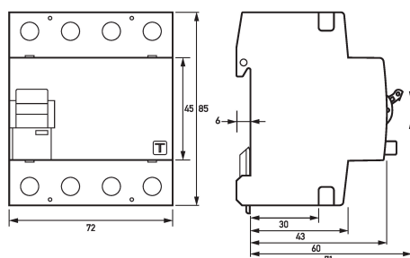
Dimensioned drawing residual current circuit-breaker DFS 4 040-4/0,03-A EV
