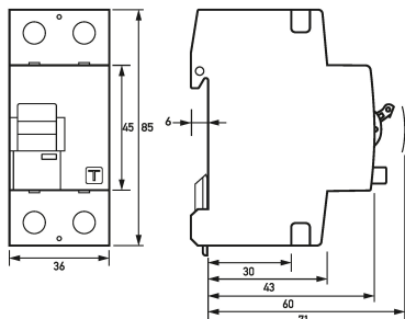
Dimensional drawing Group view
