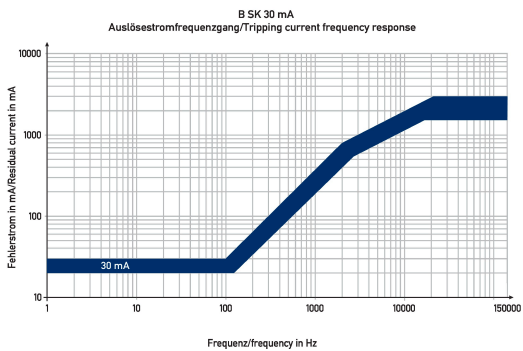
Characteristic B SK 30 mA
