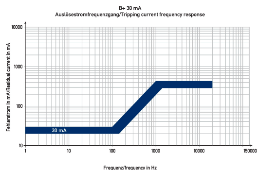
Diagrams residual current circuit-breaker DFS 2 040-2/0,03-B+ HD
